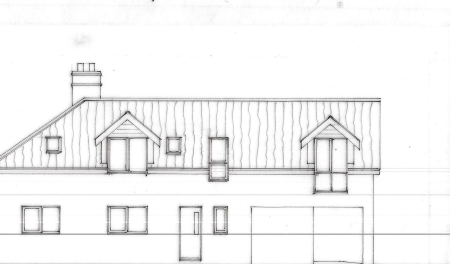
South Elevation
